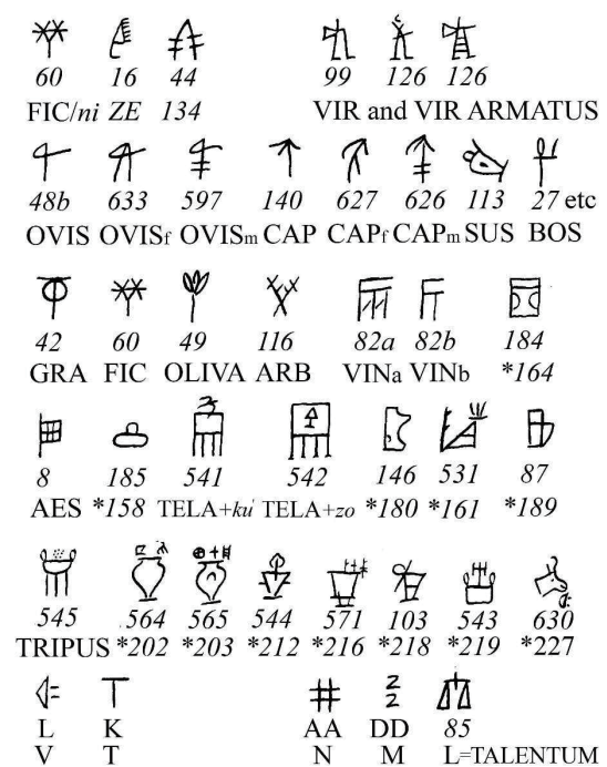
Fig. 7. Linear A ideograms with added values, signs for measures and weights resembling Linear B signs (Raison & M. Pope, 1977, p. 61)
